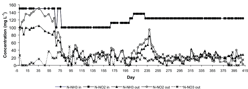
Figure 2: Nitrogen conversion in anammox reactor during the operation time
