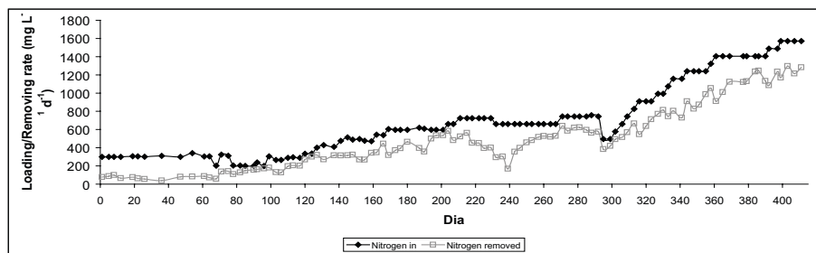
Figure 3: Nitrogen Loading/removing rate in the anammox reactor
